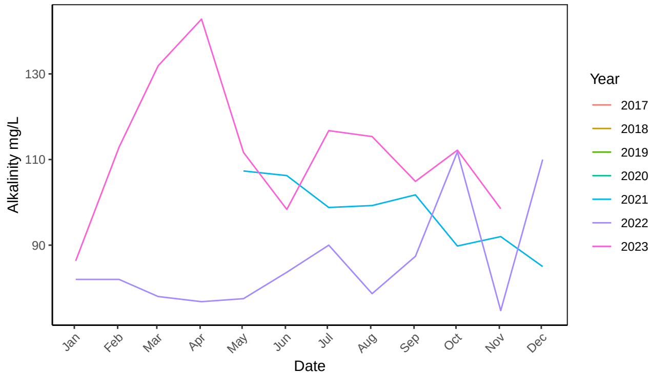
B2 Raceway 2 Alkalinity mg/L Monthly Median
